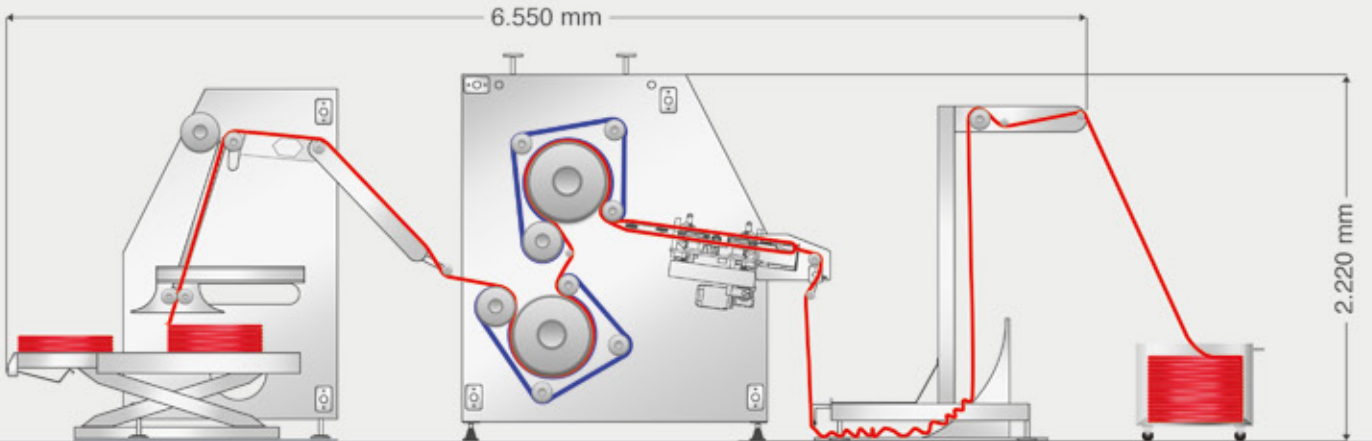
Manyetik Kumaş Eni Açma Sistemi Magnetic Fabric Width Opening System
